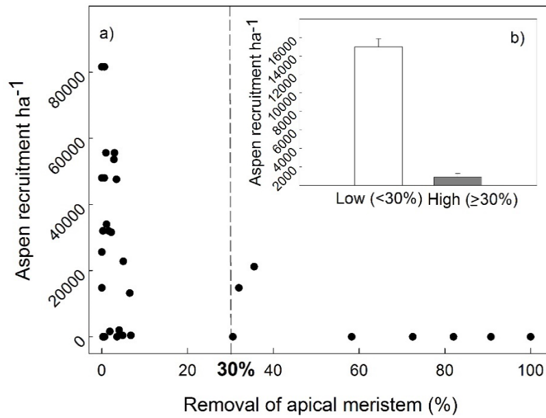
Figure 3–5. The large panel (a) shows the raw recruitment data (ha -1 ) plotted with the removal of apical meristems (%). The inset panel (b) shows the modelled recruitment data using 30% removal of apical meristems as the browse threshold. The error bar is one standard error.
