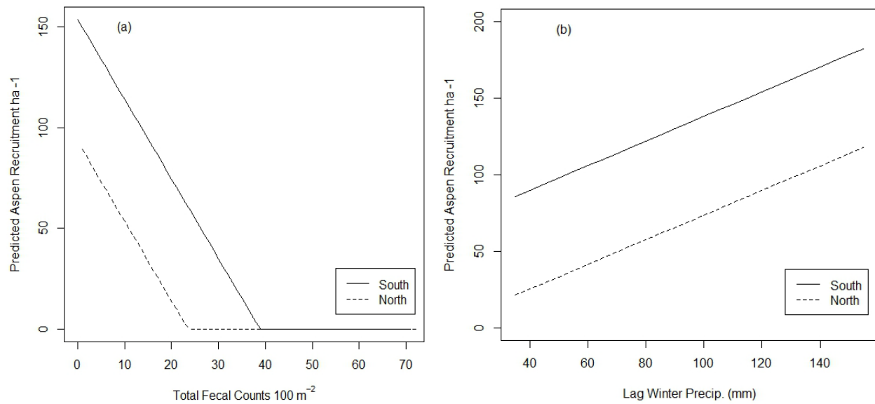
Figure 1–4. Using the zero inflation count model intercept and beta coefficients, this graph presents in panel a) the predicted mean number of aspen recruitment ( 150 \text{ cm} \leq x \leq 200 \text{ cm} ) per hectare across the observed total animal fecal counts (Cattle + Deer + Elk) and in panel b) the observed lag winter precipitation (mm). The solid line represents the predicted values at southern aspect and the dashed line represents the predicted mean at northern aspect. Lag winter precipitation was held at the mean 90 mm. Animal fecal counts (Cattle + Deer + Elk), were held at the median = 6.
